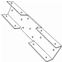
Part #23-05 2" to 3" Cross Connector
