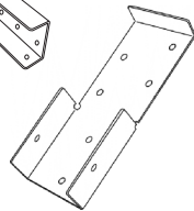
Part #23-17 2" to 3" (15") Right Rafter Connector
