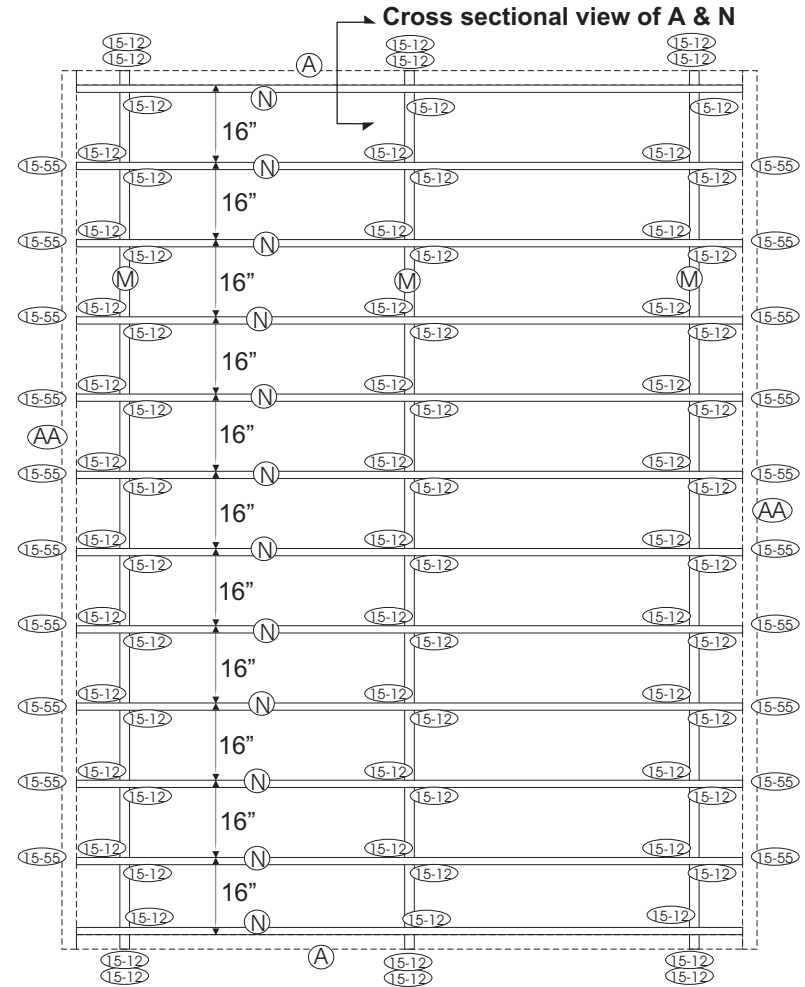
FLOOR FRAME VIEW
